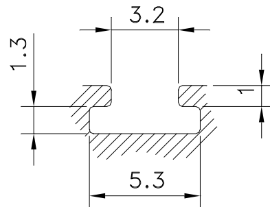
POCKET DETAILS
