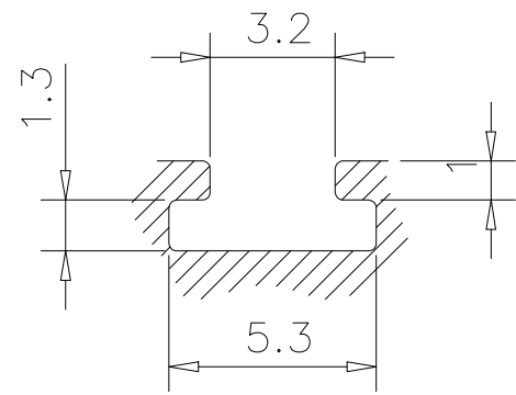
POCKET DETAILS
